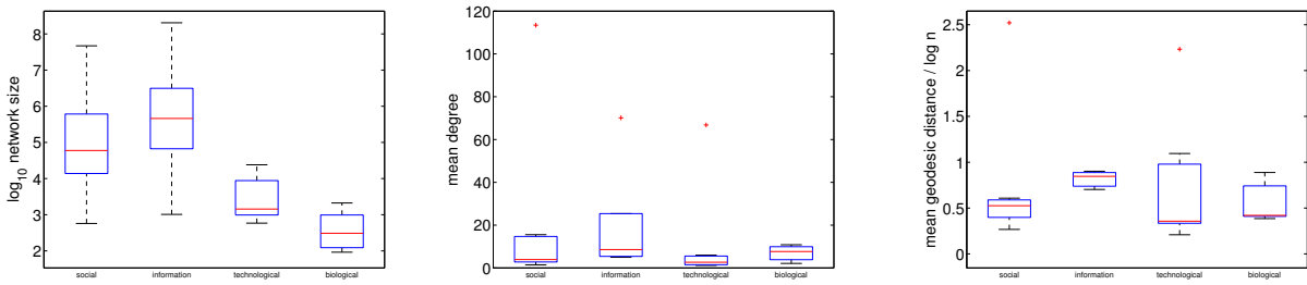
Figure 6: Boxplots showing the within-class distributions of network size ( \log n ), mean degree, and mean geodesic distance (normalized by network size).
